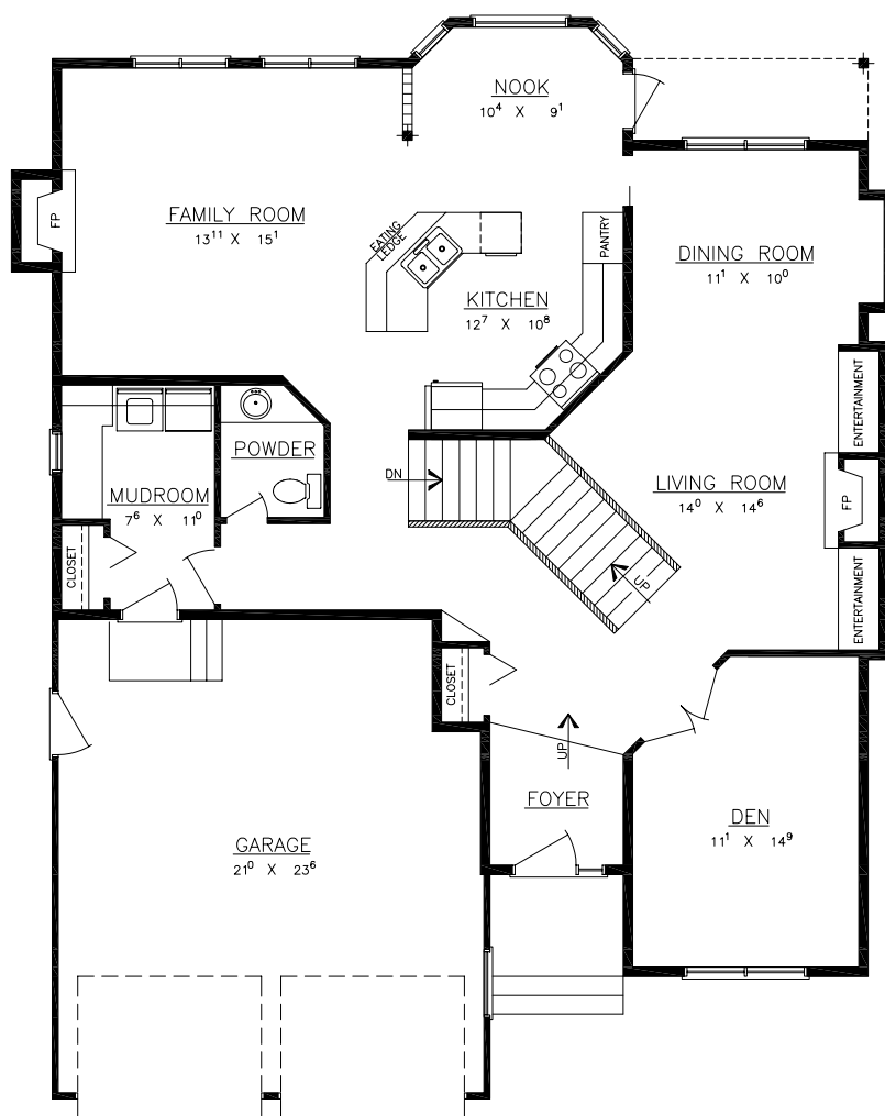
MAIN FLOOR AREA = 1416 S.F.
